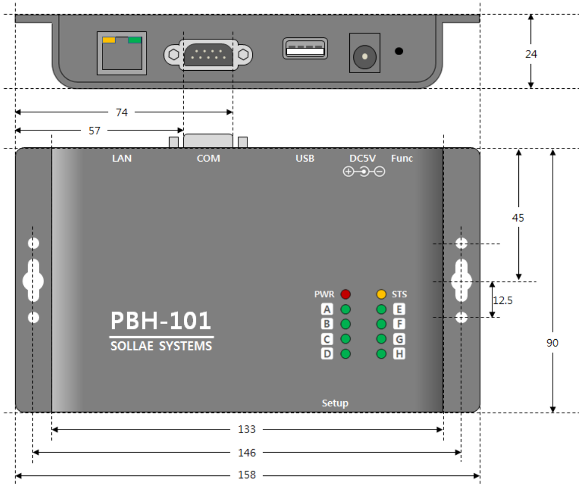
Figure 1-1 dimension
