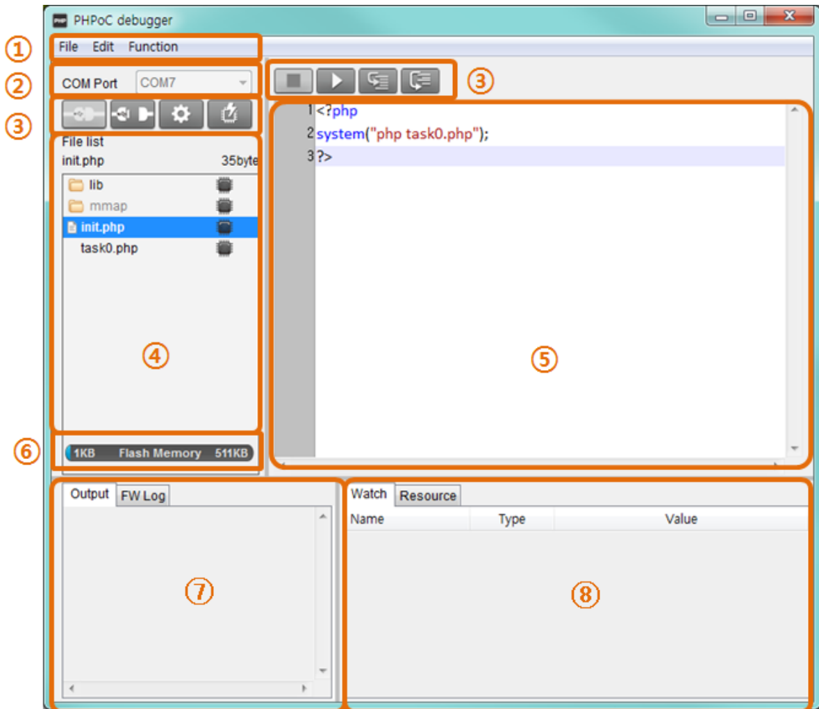
Figure 1-5 program structure
