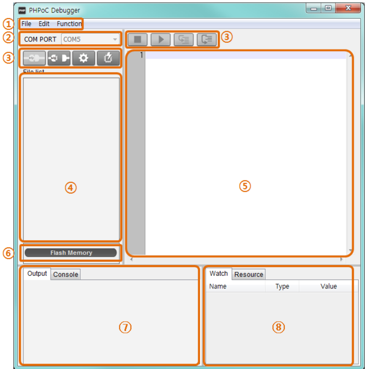
Figure 1-11 program structure
