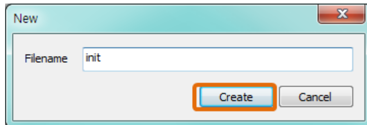
Figure 2-6 create "init.php" (2)
