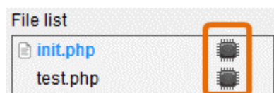
Figure 2-19 upload files
